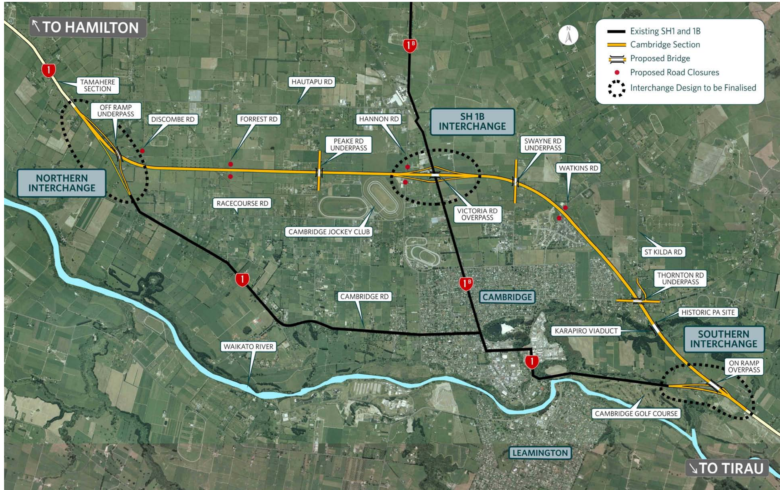
Figure 2.1 – Expressway Aerial Location Plan
