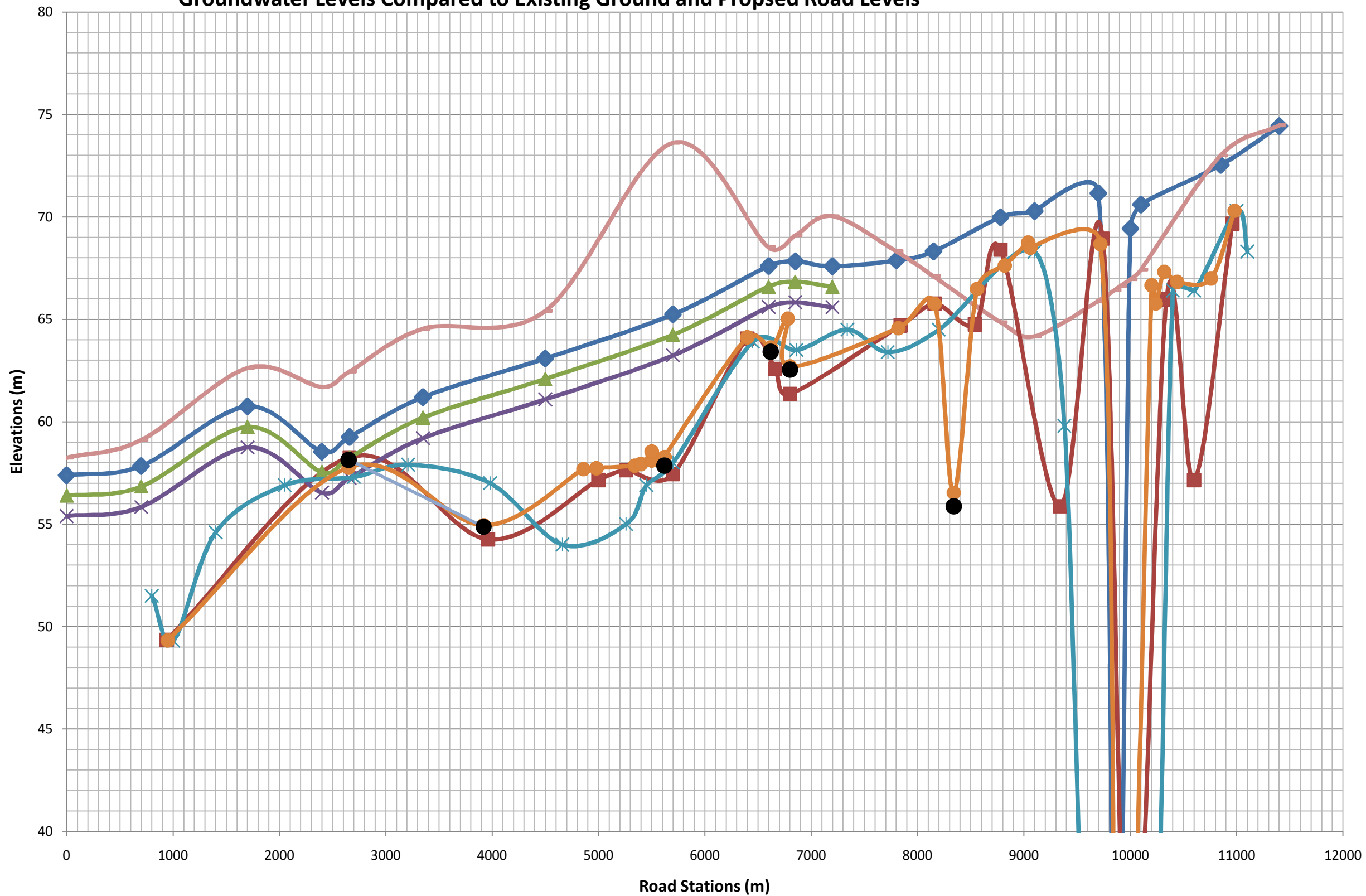
Groundwater Levels Compared to Existing Ground and Propsed Road Levels
