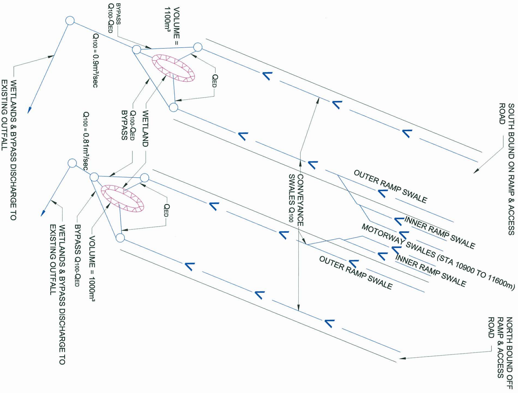
DIAGRAM OF STORMWATER SYSTEM FOR TIRAU ROAD RAMPS AND BETWEEN STATION 10900 TO 11600m
