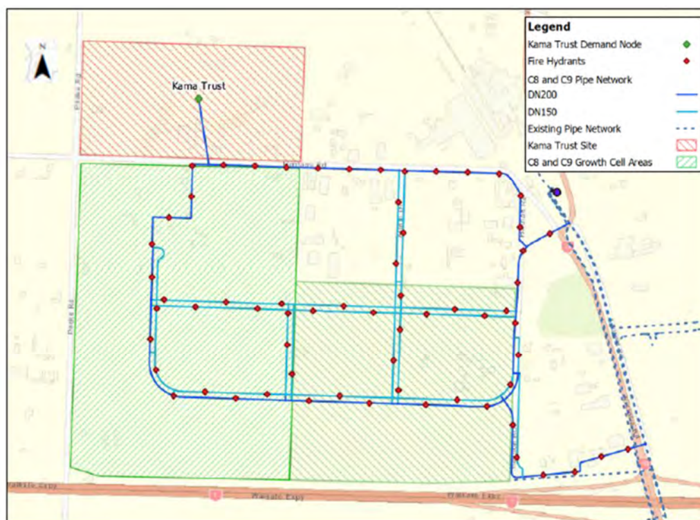
Figure 3.1: C8 and C9 Growth areas and Area 6 modelled water supply network (Appendix A)
