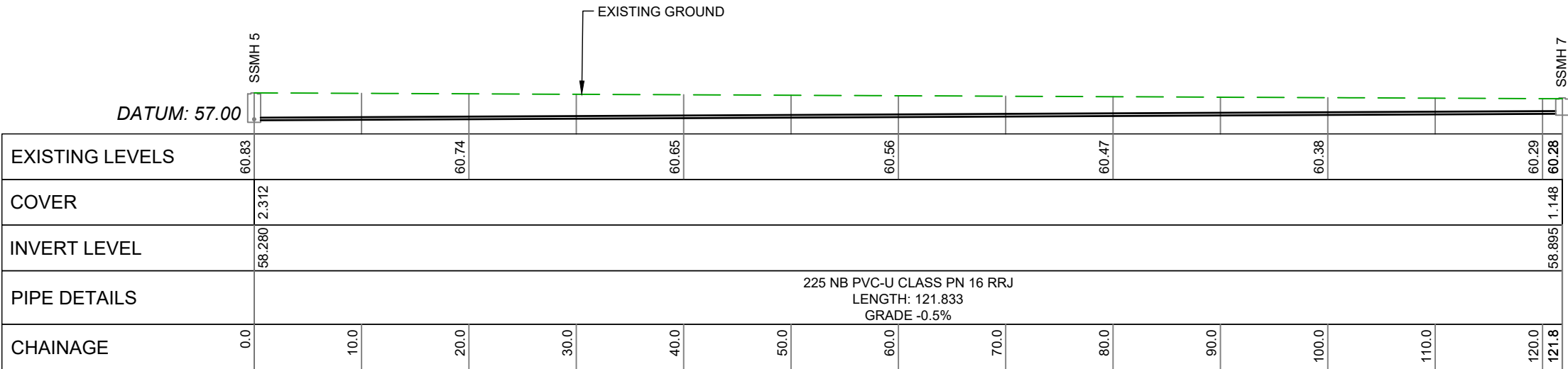
SEWER LONGSECTION (SSMH 5 - SSMH 7) SCALE 1:500
