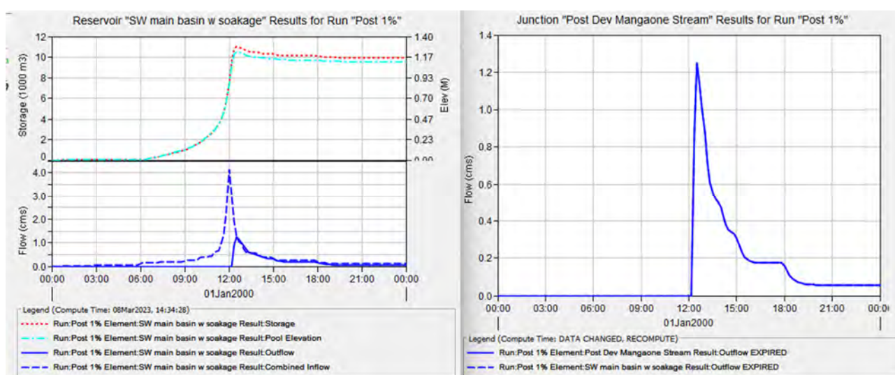
Figure D 10: Main Basin and Total Discharge to Stream, 1% AEP Design Storm Hydrograph
