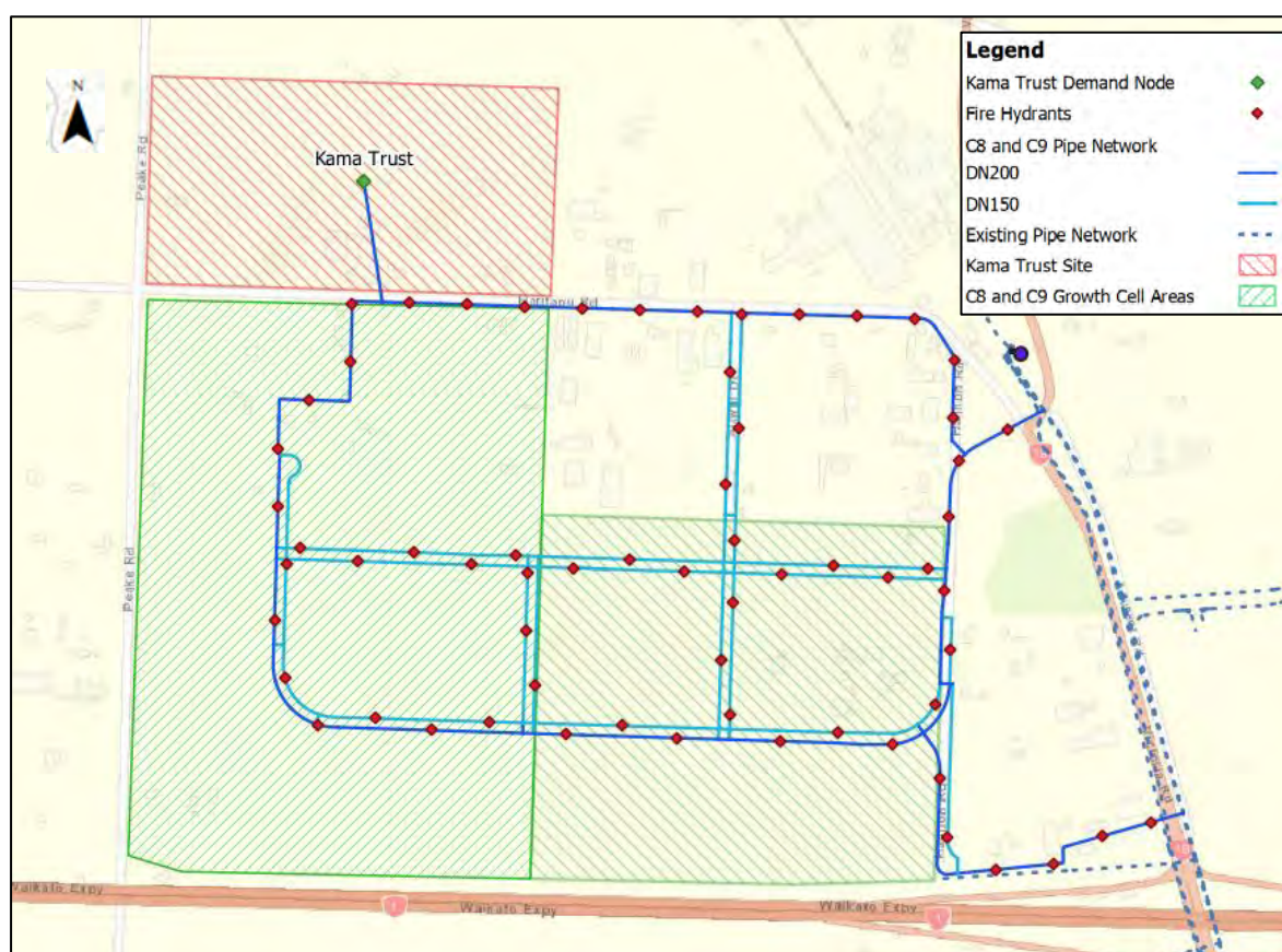
Figure 6-1: Modelled Water Supply Network
