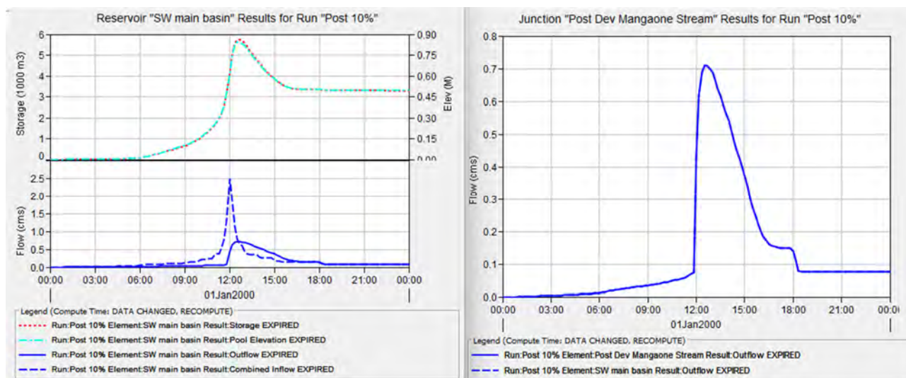
Figure C 4: Main Basin and Total Discharge to Stream, 10% AEP Design Storm Hydrograph
