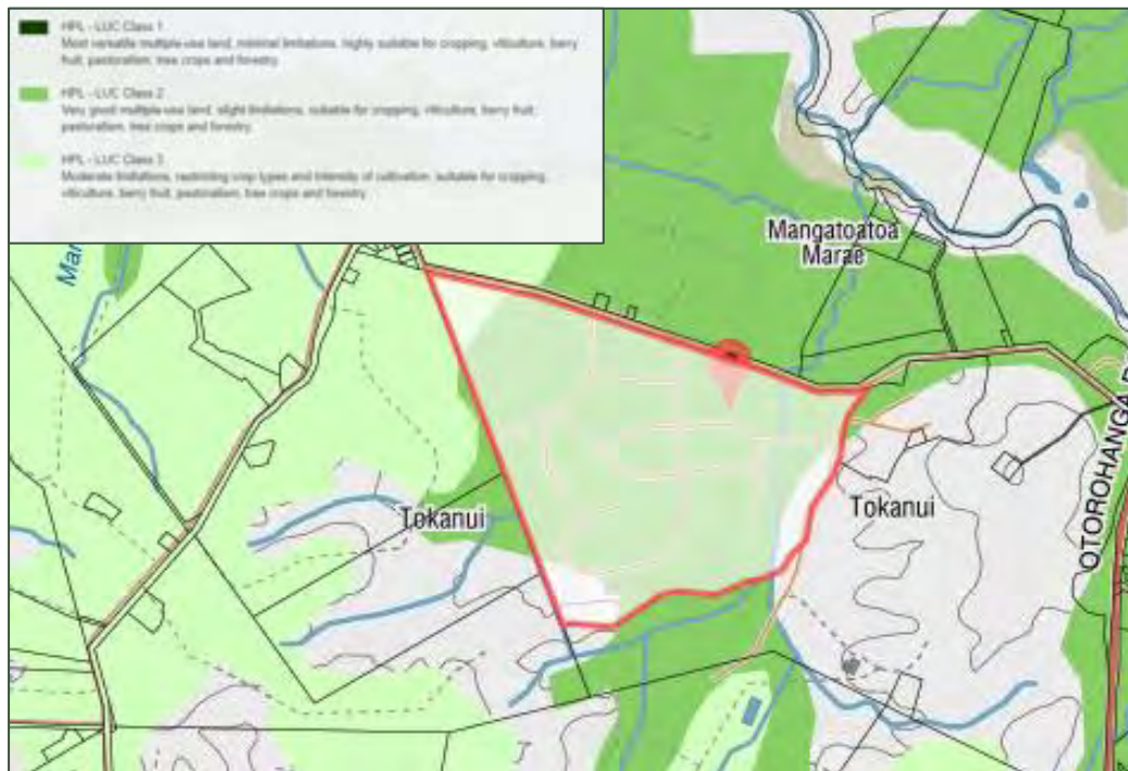
Figure 16: HPL soil classification map (Source: NZLRI)
