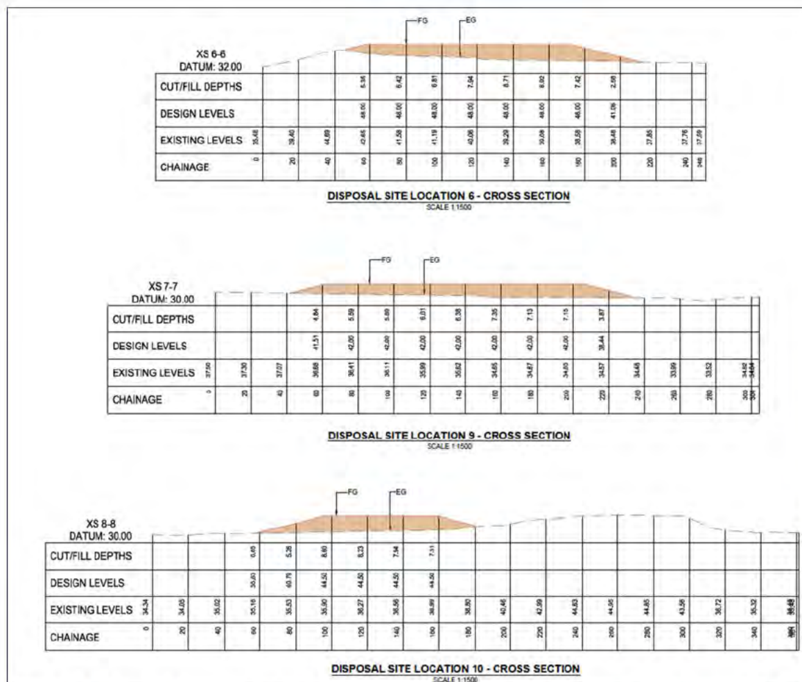
Figure 10: Potential new onsite Containment Cell Areas – Typical Cross-sections (from FTL (2023))
