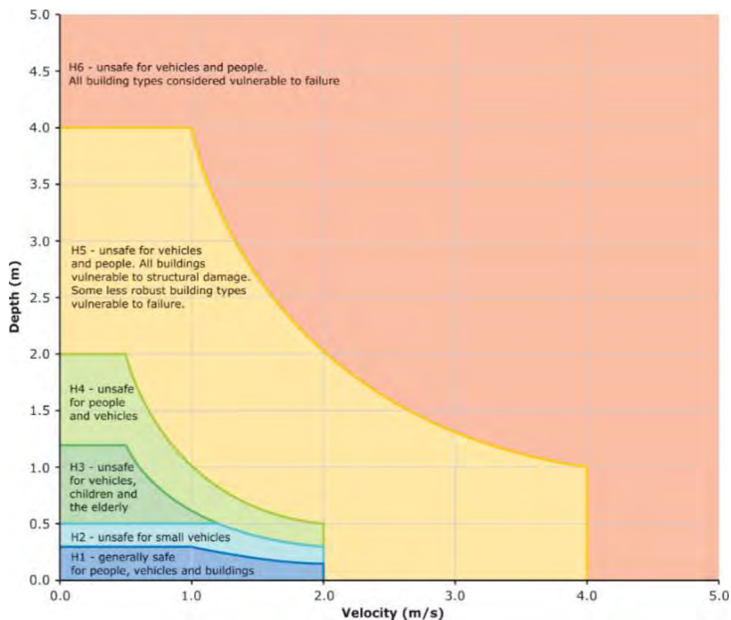
Figure 4: Depth/Velocity Envelopes (from Smith et al., 2014 – from Australian Rainfall and Runoff – Book 6: Flood Hydraulics, Chapter 7 Safety Design Criteria).
