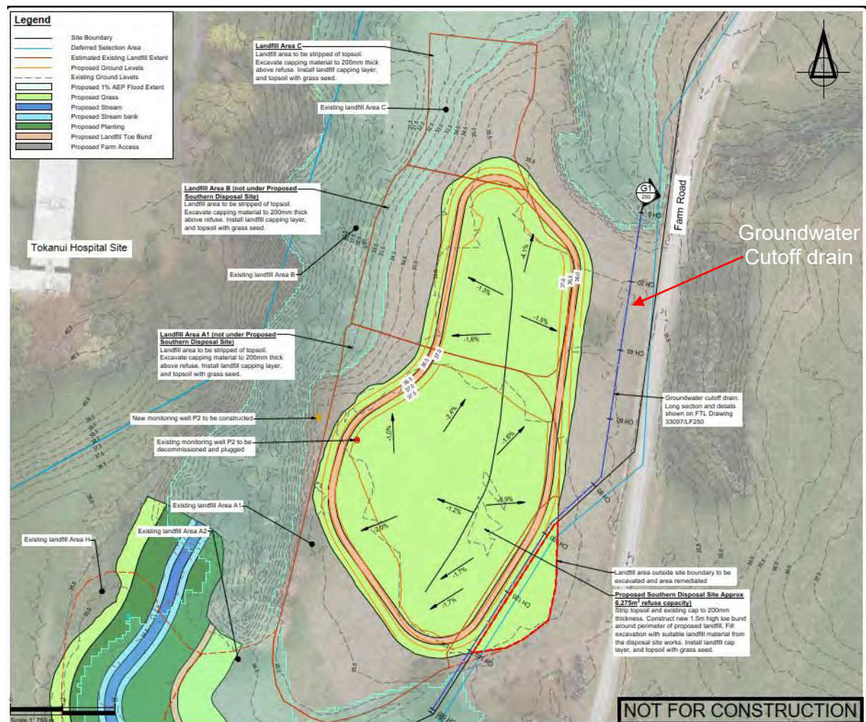
Figure 17. Area A1 showing proposed groundwater cutoff drain
