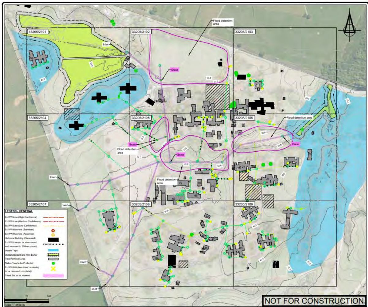
Figure 9: Stormwater infrastructure proposed to be upgraded (purple)
